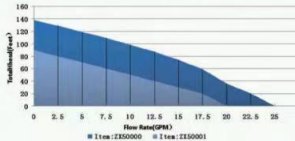
PERFORMANCE CURVES
