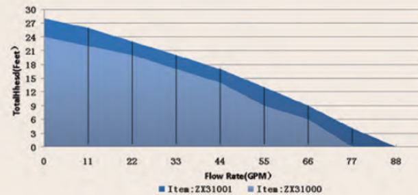
PERFORMANCE CURVES
