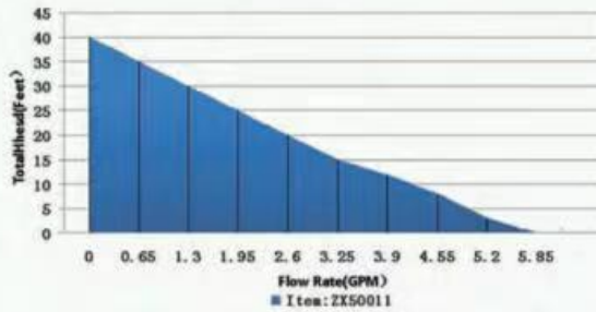
PERFORMANCE CURVES
