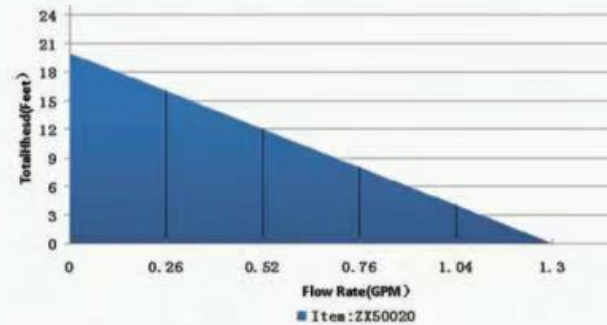
PERFORMANCE CURVES
