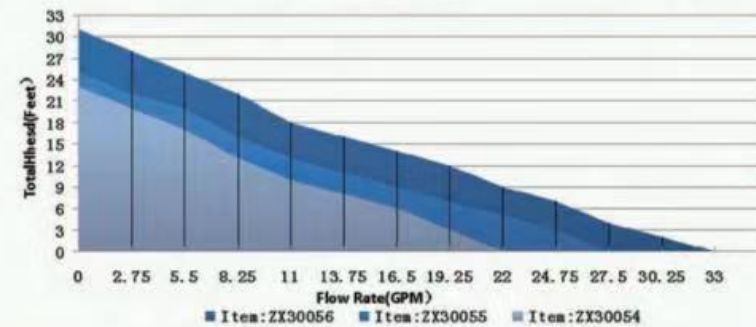
PERFORMANCE CURVES
