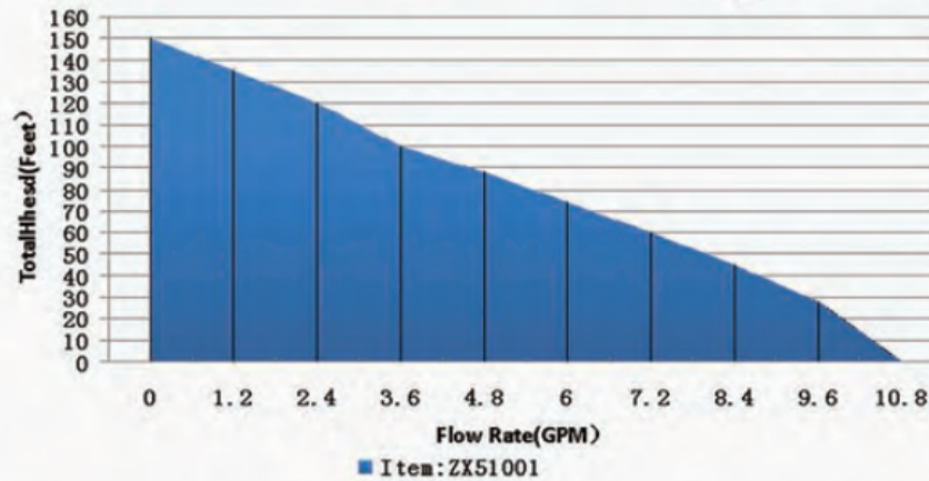
PERFORMANCE CURVES
