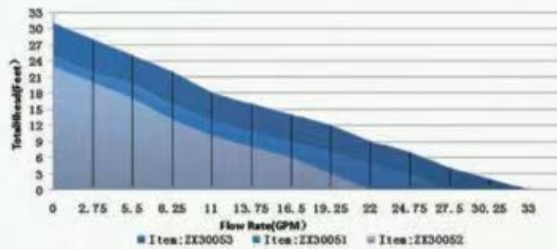
PERFORMANCE CURVES
